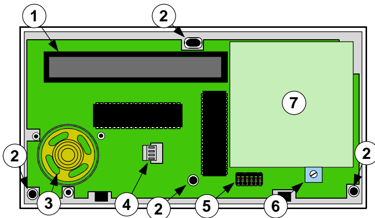
Figure 1: D1256/D1257 Internal Arrangement
